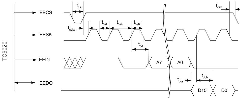
FIGURE 13: EEPROM Switching Characteristics
