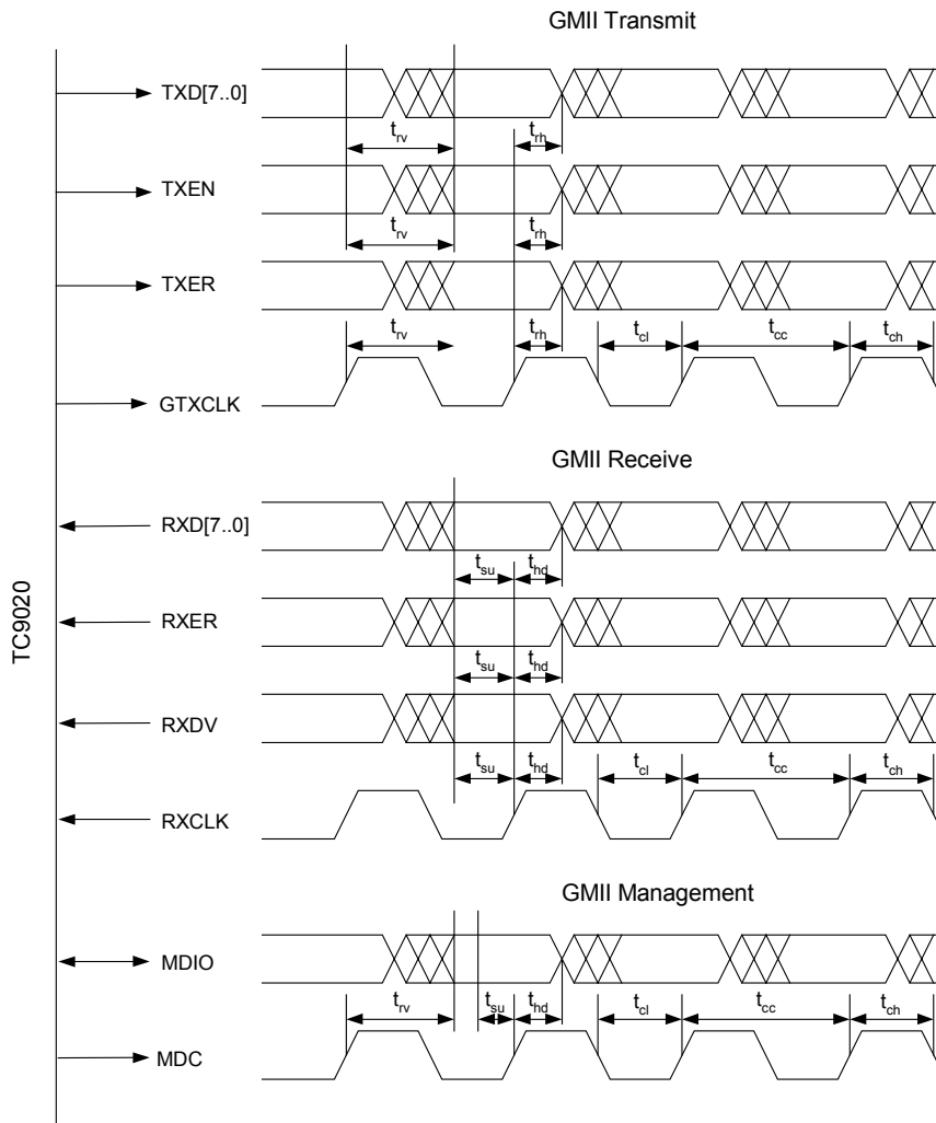
FIGURE 14: GMII Switching Characteristics
