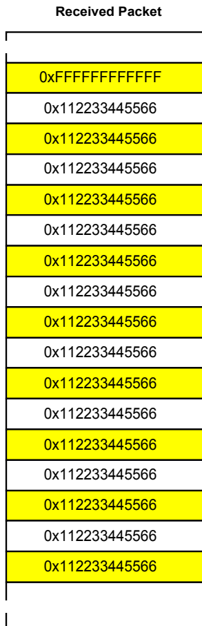
FIGURE 7: Example Magic Packet
