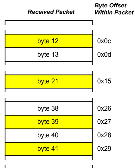
FIGURE 6: Example Wake Packet
