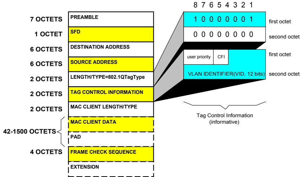
FIGURE 10: VLAN Tag Format from IEEE 802.3 Standard.
